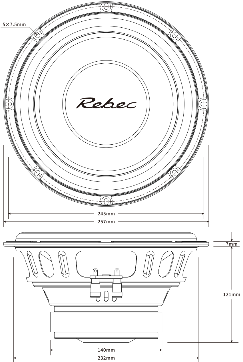
Speaker Dimension Drawing
