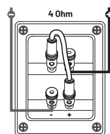
- Serial connection - - with jumpers -
