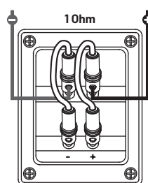
- Parallel connection - - with jumpers -
